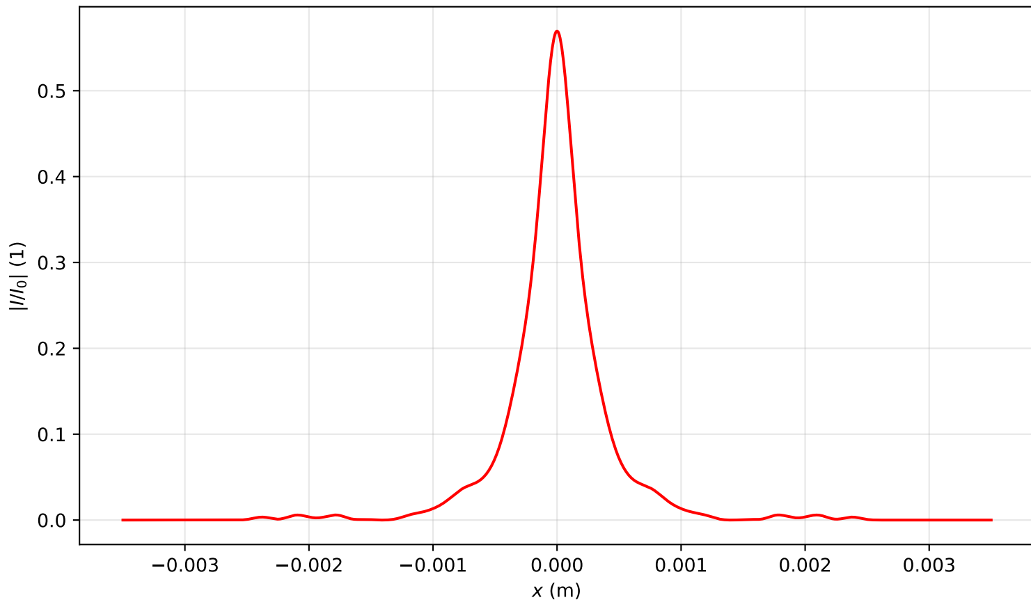
Intensity profile I(x, y = 0, z = 2.548)/I_0 , P_{in}=4.0P_{cr} , artificial time
